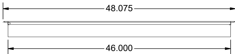
BLRE 4' 6"W H25, Side View
